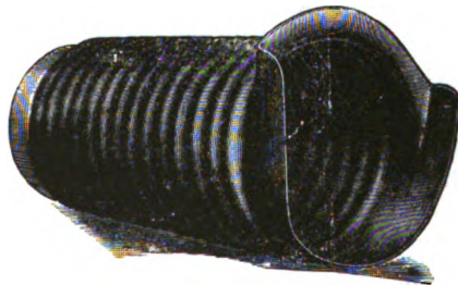
FIG. 76.—FORM OF CORRUGATED FLUE USED AS FURNACE IN MARINE BOILER.
